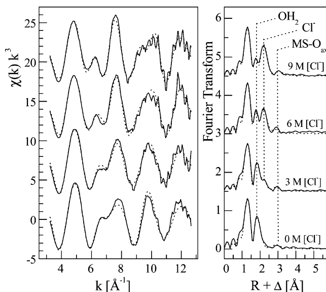
Figure 2. U L III -edge k^3 -weighted EXAFS data (left) and corresponding Fourier transforms (right) taken over k = 3.2 – 12.7 \text{ \AA}^{-1} for \text{UO}_2^{2+} as a function of [\text{Cl}^-] : experimental data (line); theoretical curve fit (dots).
